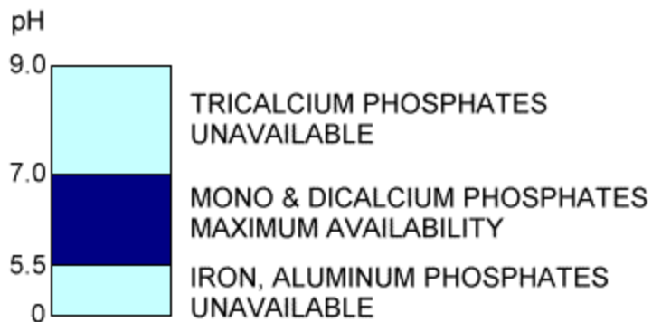
Figure 6.2 Soil pH Affects Phosphorus Availability
